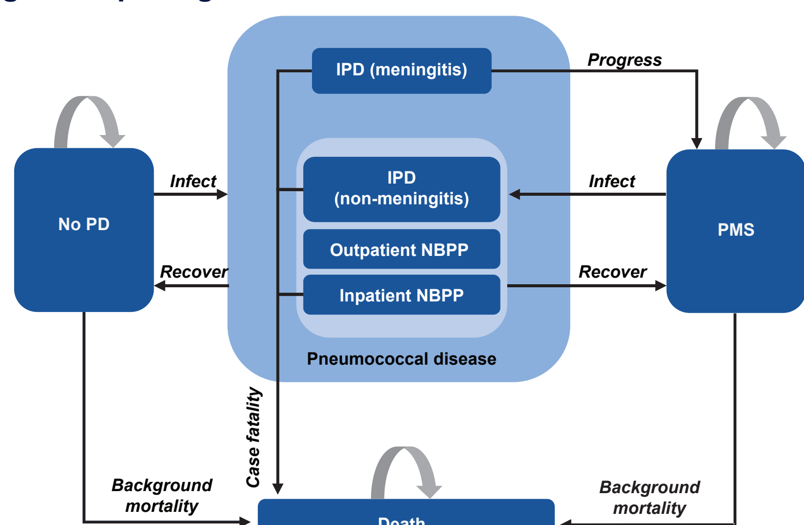
Figure 1. Schematic diagram depicting the structure of the state-transition Markov model
